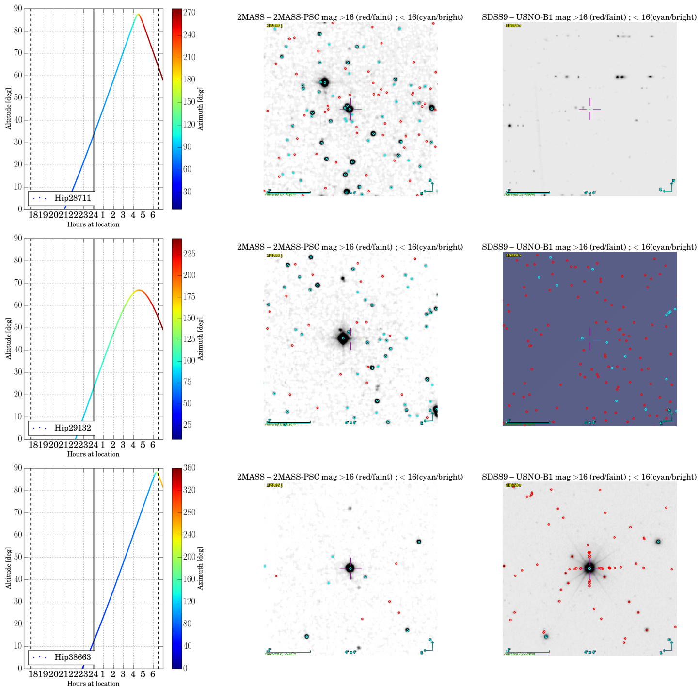
Figure 6: con't LUCI/IRTC stars.
