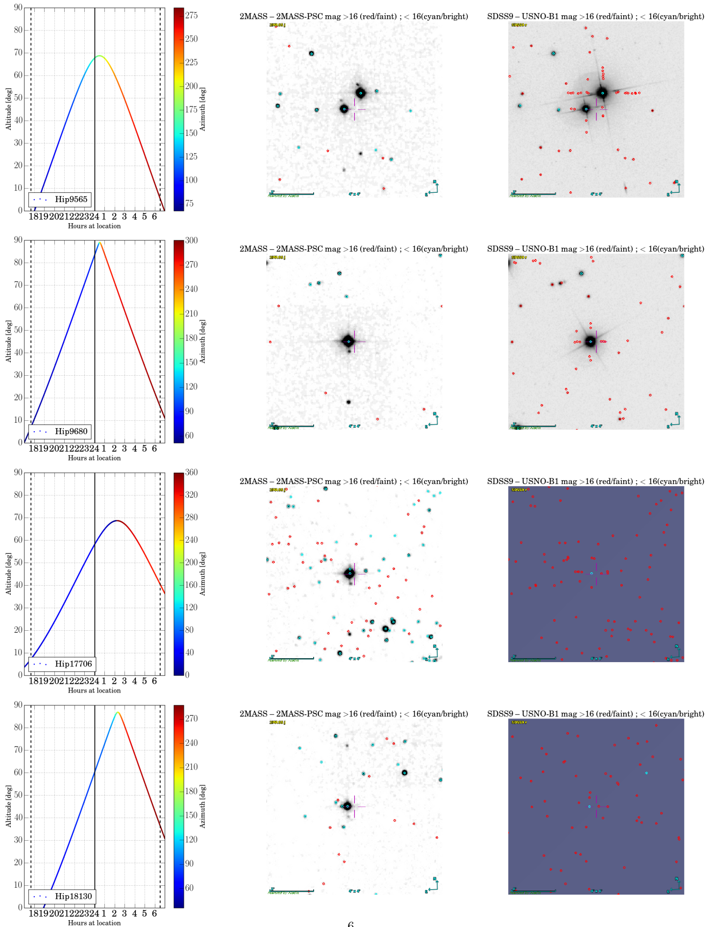
Figure 5: con't LUCI/IRTC stars.
