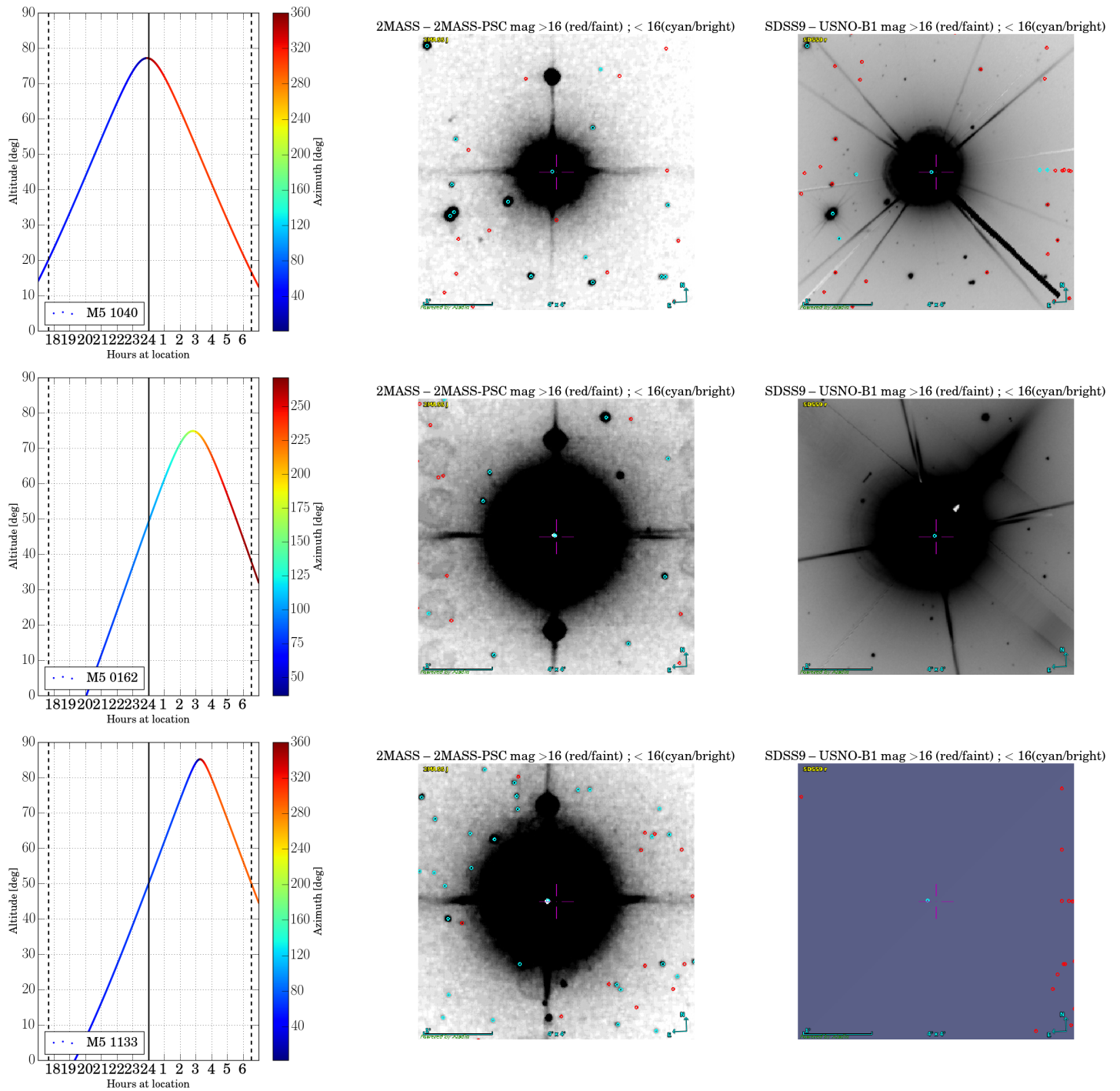
Figure 3: con't Bright stars
