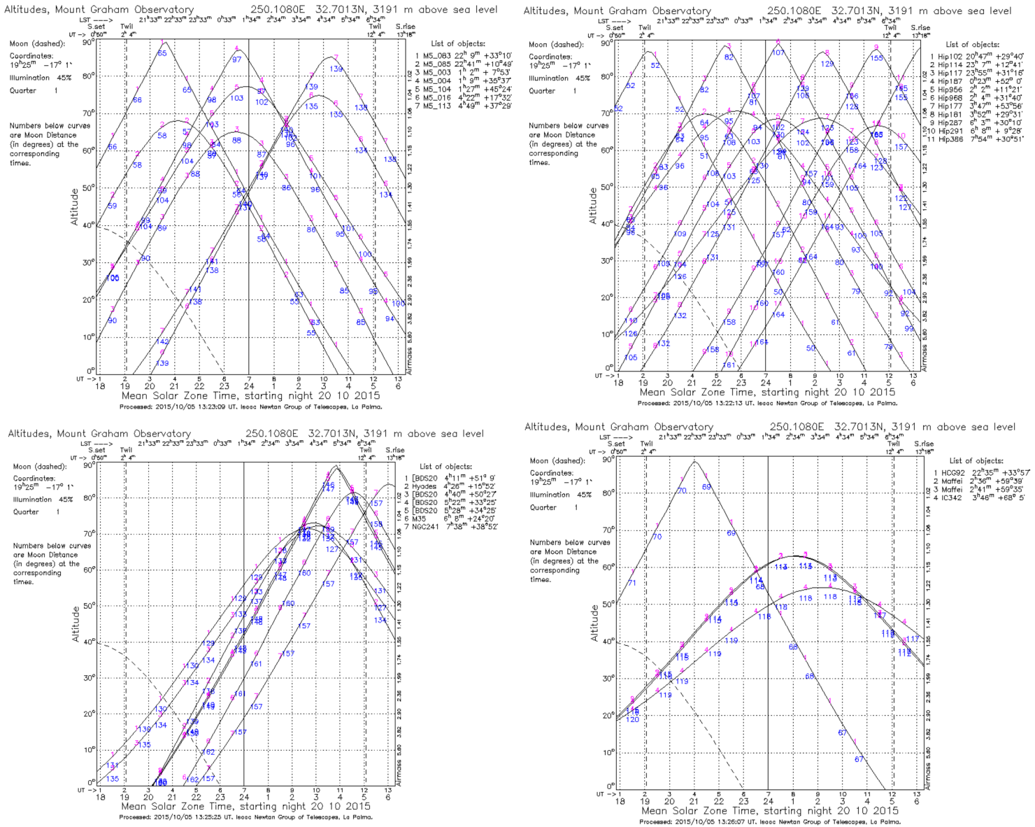
Figure 1: (Top Left) Bright stars. (Top Right) Technical targets. (Bottom left) star cluster targets. (Bottom right) Additional MPIA targets.
