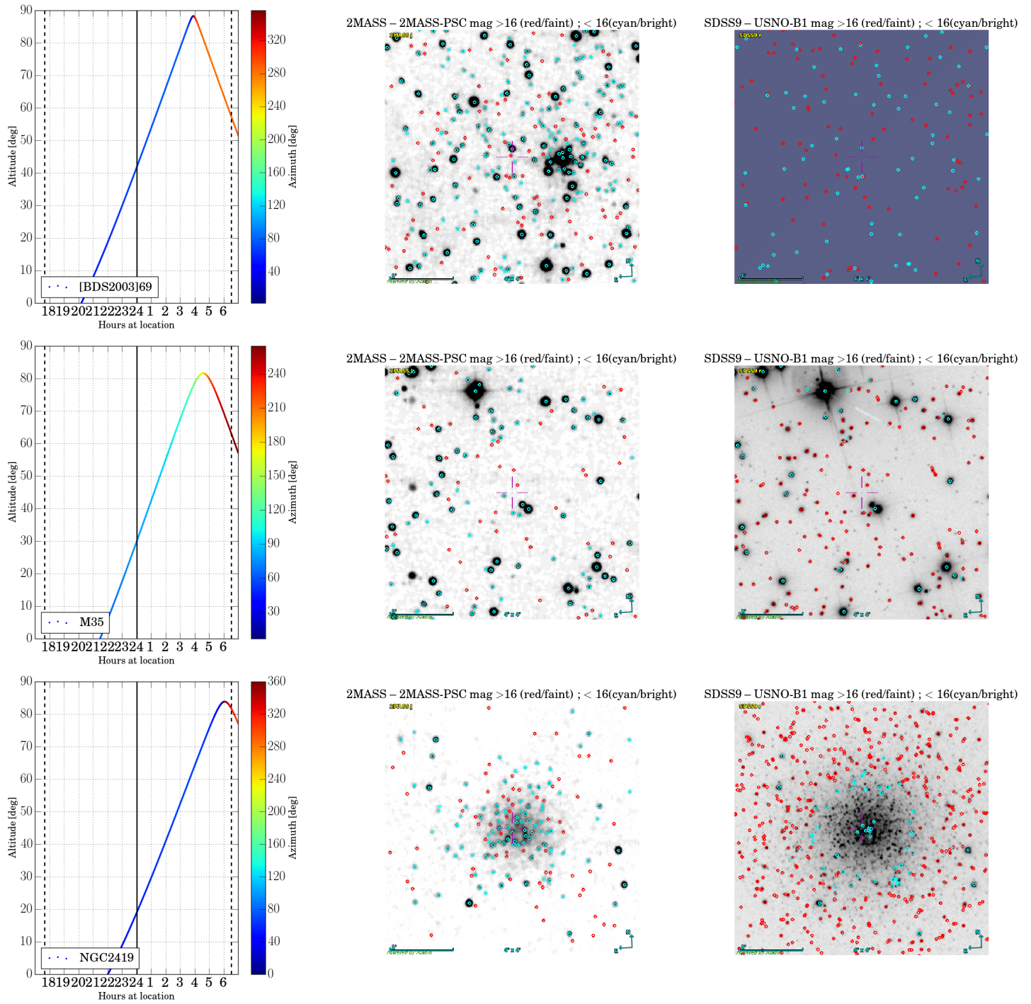
Figure 8: con't star clusters.
